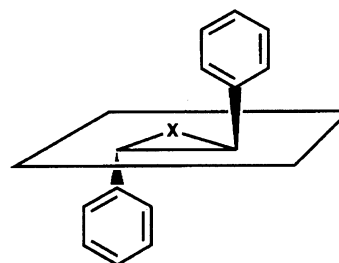
Fig. 7. Conformation of the enantiomers of 9 and 14 adsorbed more strongly to 1a .
